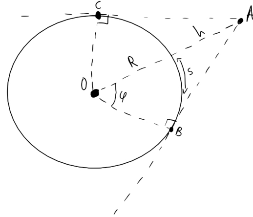
Figure. 1 Horizon geometry. S is the arc length along the Earth's surface to the horizon point, R is the radius of the Earth, and h is the observer's altitude above the surface. The quantity \arccos(R / (R + h)) is the central angle \phi between the observer and the tangent point, measured in radians.
