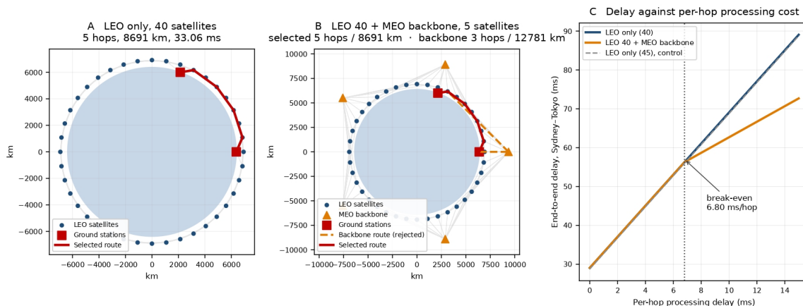
Figure. 4 Controlled comparison of end-to-end delay with and without a MEO backbone. All panels route between identical ground stations at the Sydney to Tokyo central angle of 70.38^\circ , corresponding to 7,826 km great-circle distance, over an identical LEO stroma of 40 satellites at 550 km. A. LEO-only configuration: the selected route uses 5 hops over 8,691 km for a total modelled delay of 33.06 ms. B. The same stroma with a five-satellite MEO backbone at 3,000 km. The router still selects the LEO route, shown solid; the backbone route, shown dashed, reaches the destination in 3 hops but traverses 12,781 km. C. Total end-to-end delay against per-hop processing delay for both configurations, with a control in which the five additional satellites are placed in LEO. The curves cross at 6.80 ms per hop. Generated by make_figure4.py, commit 405d8fe.
