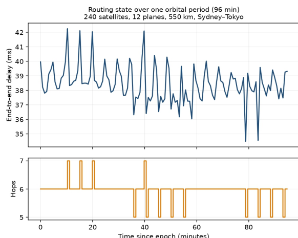
Figure. 5 Routing state over one orbital period. A constellation of 240 satellites in 12 planes at 550 km, routing between Sydney and Tokyo, sampled at 120 epochs across one orbital period of 95.5 minutes. The connectivity graph is rebuilt from scratch at each epoch. Upper panel, end-to-end delay; lower panel, hop count. Generated by make_figure5.py , commit 405d8fe.
