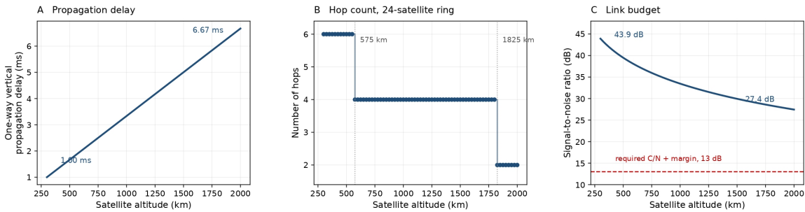
Figure. 2 Relationship between satellite altitude and network variables. A. One-way vertical propagation delay against altitude, 300 to 2,000 km. B. Simulated hop count against altitude for a 24-satellite ring, 2,500 km inter-satellite link range, endpoints 60^\circ apart, 10^\circ elevation mask. Markers are simulated values; hop count is integer-valued and changes at 575 km and 1,825 km. C. Signal-to-noise ratio against altitude in dB, with the 13 dB required carrier-to-noise ratio and margin marked. Generated by make_figure2.py, commit 405d8fe.
