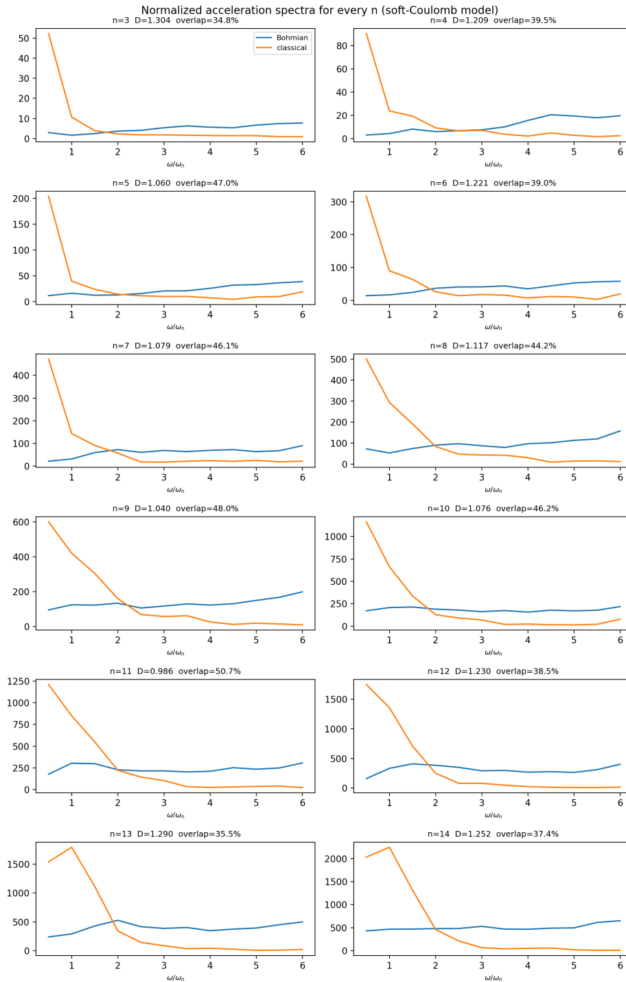
Figure. 5 Normalized Bohmian (blue) and Classical (orange) ensemble-averaged spectra for n from n = 3 to n = 14 .
