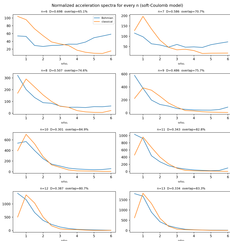
Figure. 6 Spectra of Bohmian (blue) and classical (orange) ensemble-averaged spectra for \bar{n} ranging from 6 to 13.
