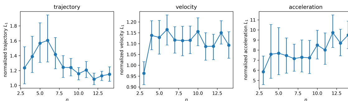
Figure. 4 The L_1 motion difference metrics for family A.
