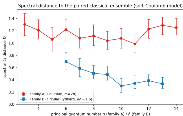
Figure. 3 The spectral distance metric for both families A and B.
