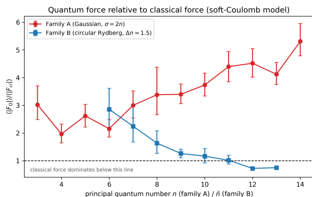
Figure. 2 The quantum force ratio for both families, as n increases
