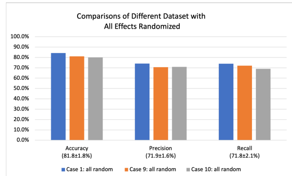
Fig. 3 Comparisons of Cases 1, 9, 10 with all effects randomized for 1000 randomized sentences on three groups of prediction analysis data. Mean±SD (standard deviation) for these three groups of data are shown.
