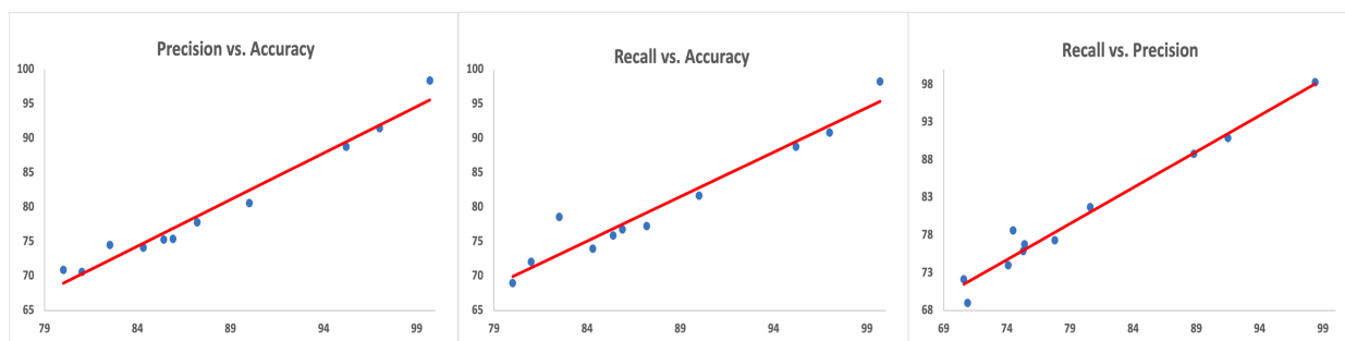
Fig. 4 Correlation diagrams among accuracy, precision, and recall data for all datasets.
